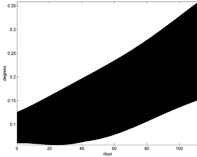
Figure 4.13: Difference in angle from the earth's center.
