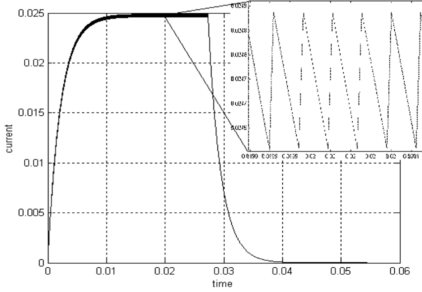
Figure 4.20: PWM controlled current in RL circuit
