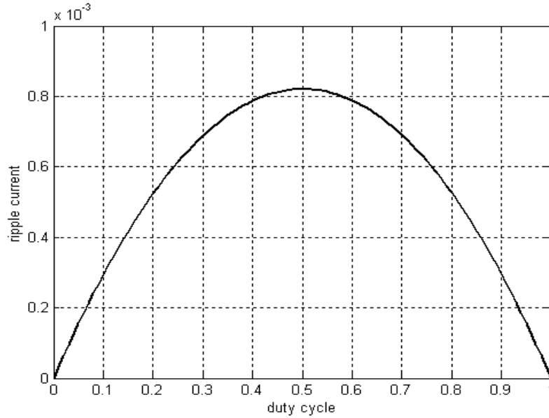
Figure 4.18: Ripple current as a function of duty cycle.
