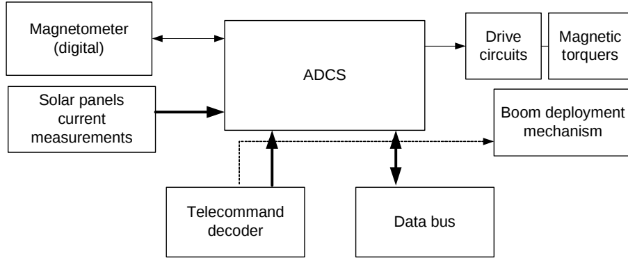
Figure D.1: ADCS block diagram
