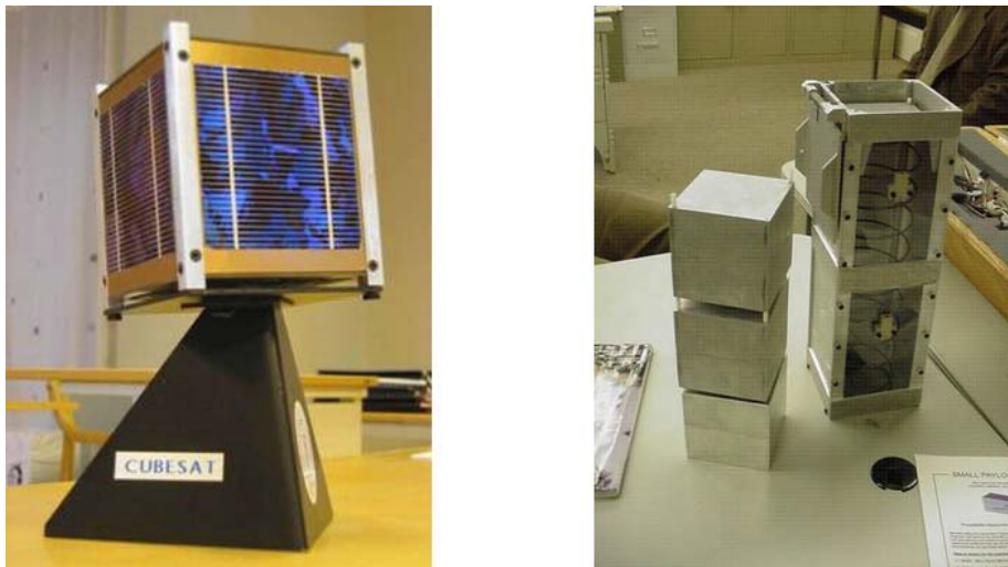
Figure 1.1: The NCUBE cubesat and the cubesat launcher
