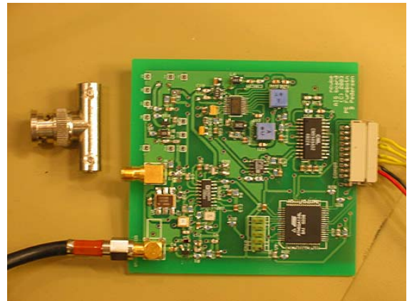
Figure 5. Miniaturized AIS VHF receiver.
