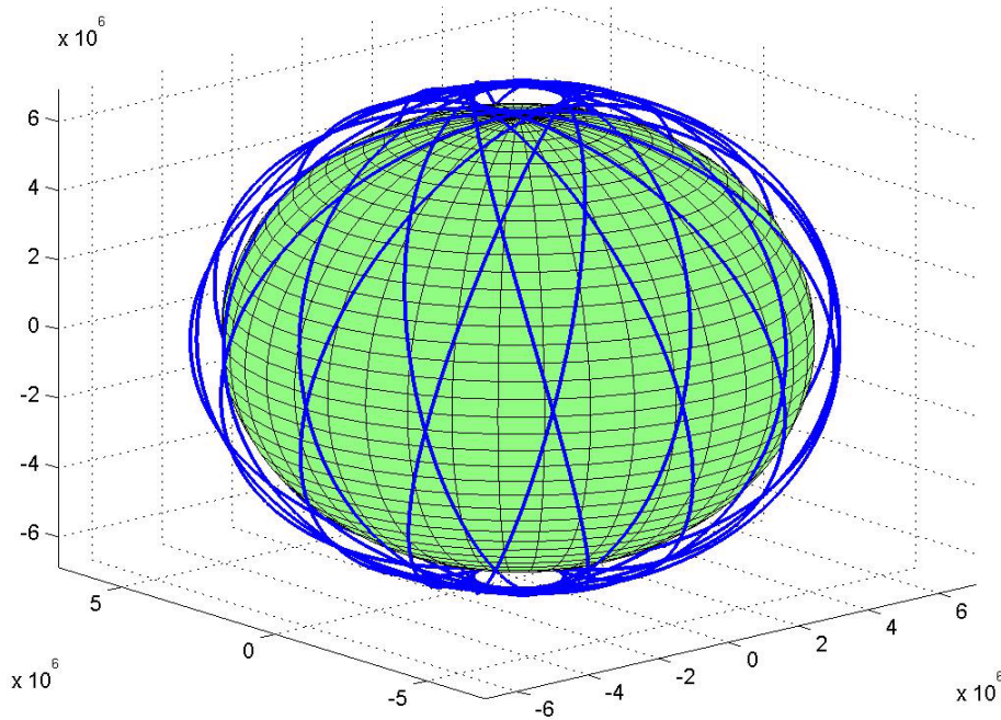
Figure 4.6: The earth with satellite track
