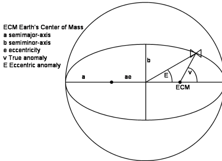
Figure 4.8: The keplerian elements in plane
