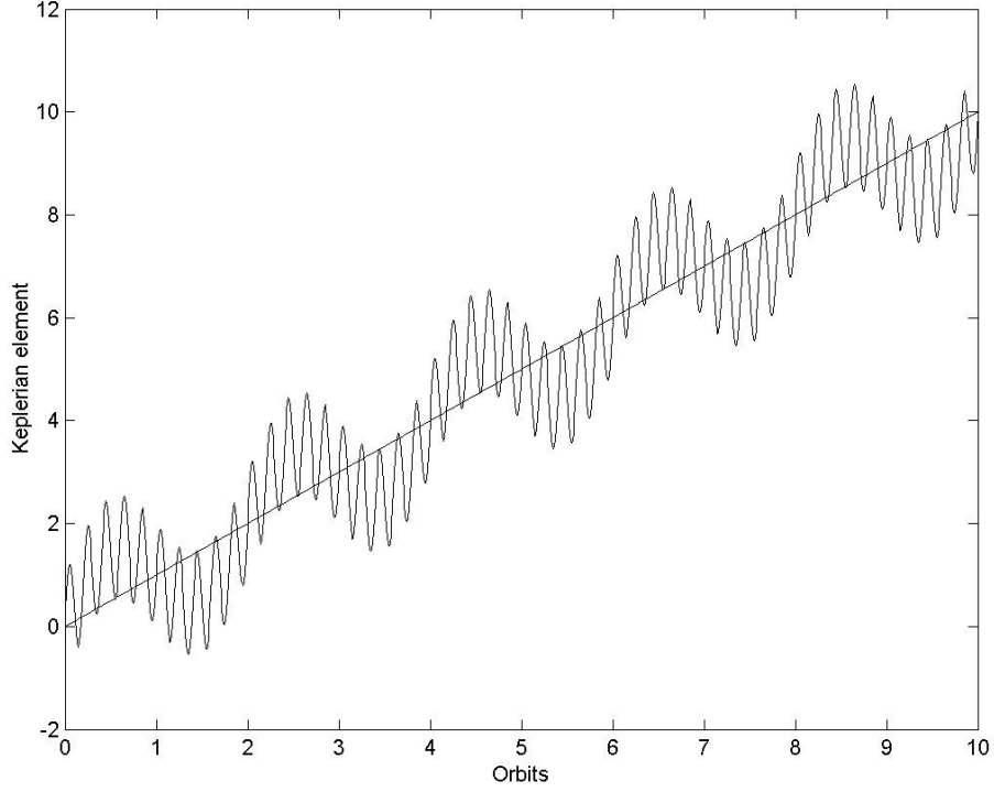
Figure 4.11: The perturbations of a keplerian element
