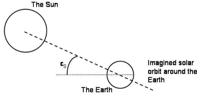
Figure 4.5: The sun's imagined orbit around the earth.
