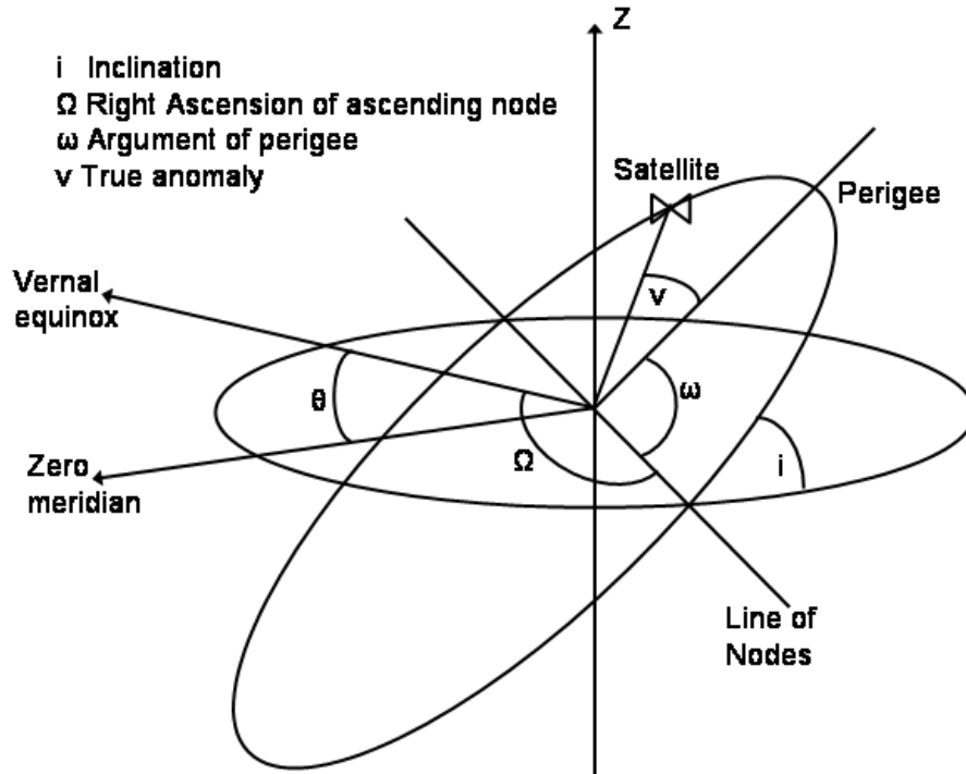
Figure 4.7: The keplerian elements
