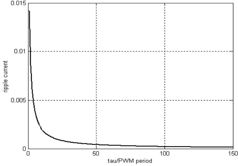
Figure 4.19: Ripple as a function of PWM frequency
