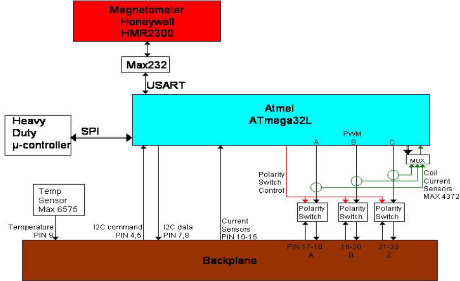
Figure 6.1: NCUBE ADCS block diagram
