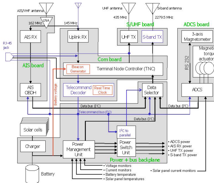
Figure 1.2: The NCUBE system architecture
