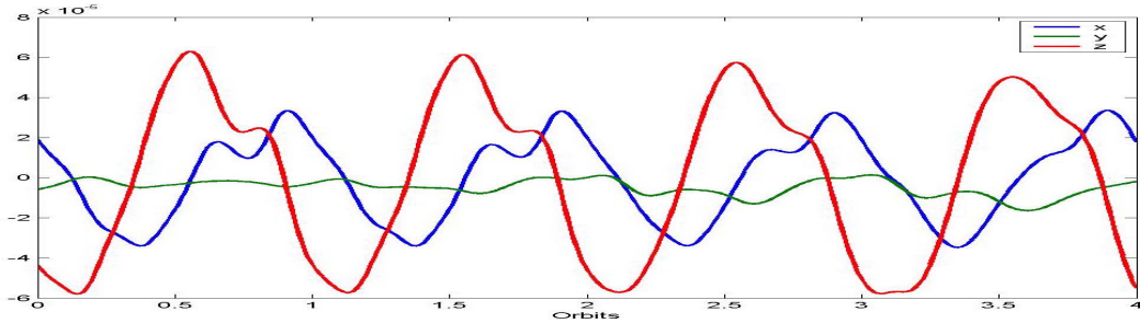
Figure 4.15: The earth's magnetic field from IGRF model
