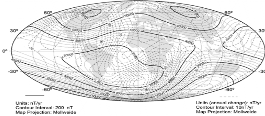
Figure 4.14: Magnitude of the earths magnetic field.
