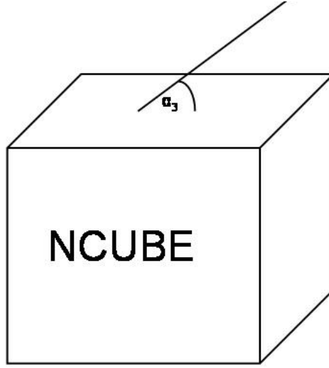
Figure 4.4: Sunbeam 3D angle of attack
