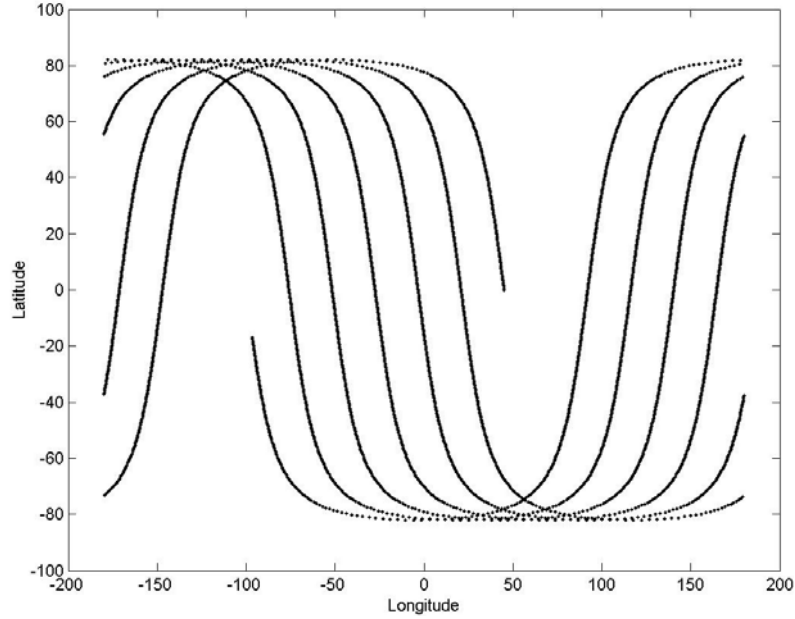
Figure 4.10: Simple orbit propagation
