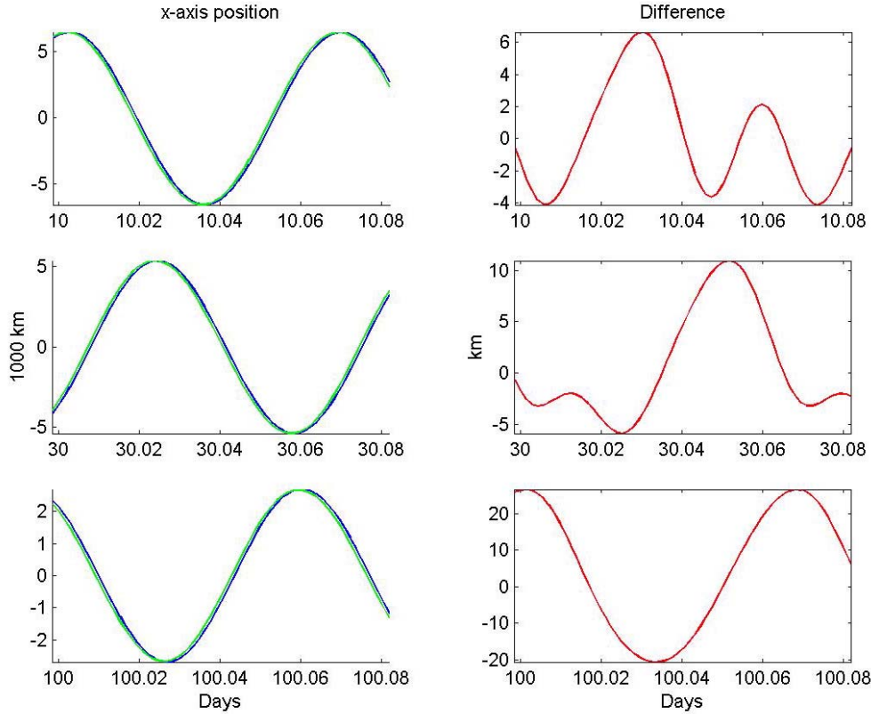
Figure 4.12: Estimates made by the SGP4 and the enhanced simple orbit estimator.
