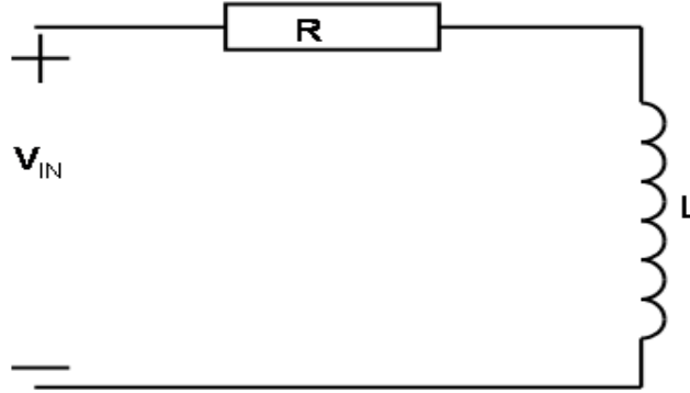
Figure 4.17: The RL circuit representing the magnetic coil
