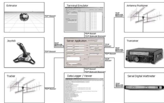
Figure 6. Ground station system overview.
