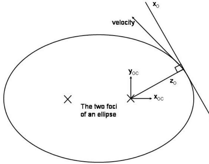
Figure 3.1: The difference between the velocity and a normal to a vector from a focus
