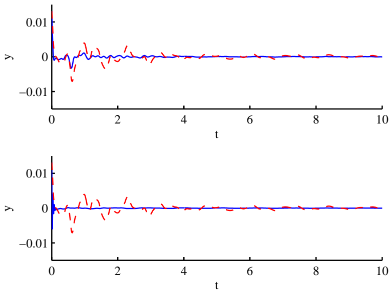
Figure 4.3: Performance with robust MPC (top) and NMPC (bottom) The open loop response is shown as the red, dashed line.
