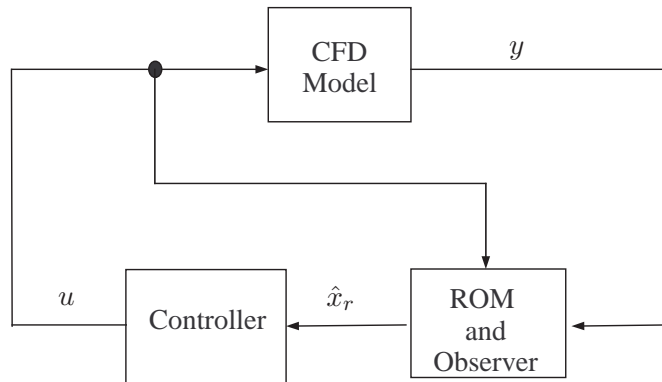
Figure 2.4: Block diagram of the reduced-order output-feedback setup. \hat{x}_r is an estimate of the reduced state based on an observer, using the reduced model (ROM) and measurements from the CFD model.
