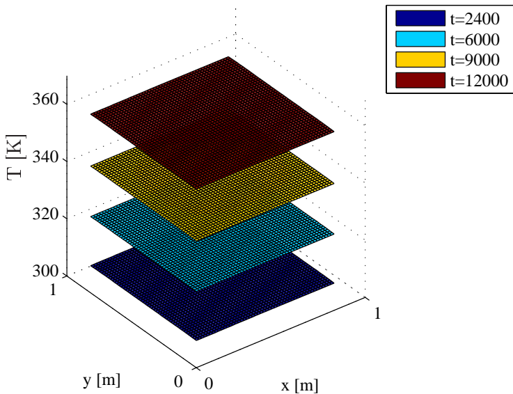
Figure 2.7: Plate temperature without control, shown for t = 2400, 6000, 9000 and 12000 s.
