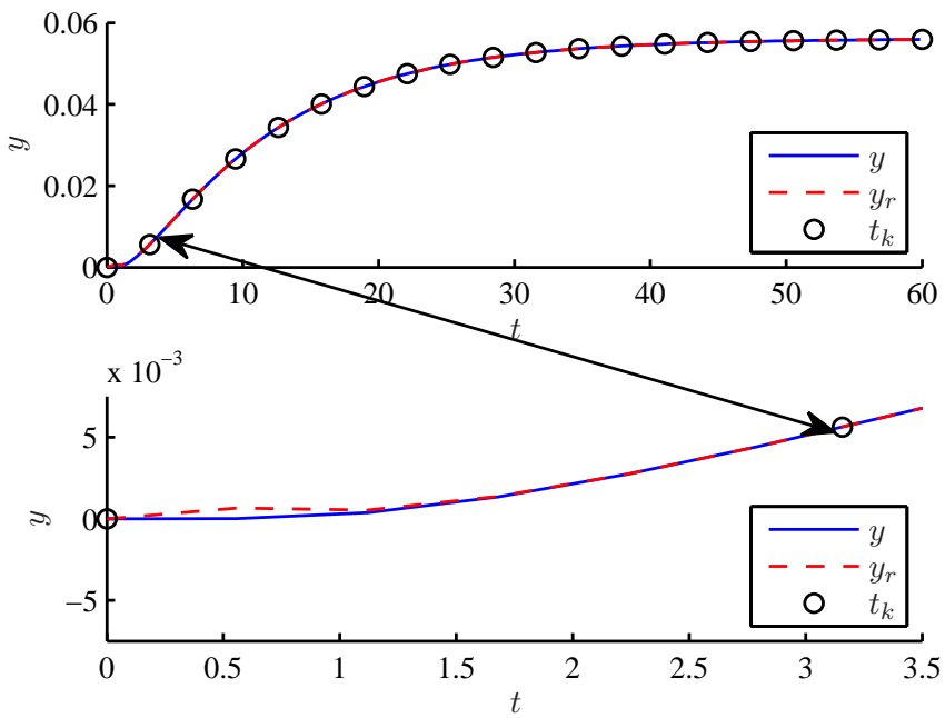
Figure 5.1: Step response of high-fidelity model and reduced-order model of order r = 4 , generated using 20 snapshots uniformly distributed between 0 and 60s. The transient error is emphasized by zooming in the bottom plot.
