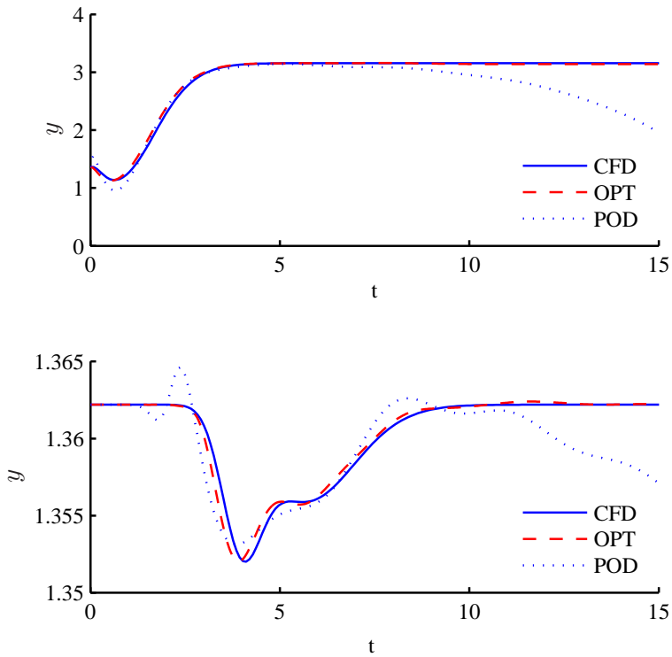
Figure 5.11: Top: Response in Mach number y to step in bleed input b for the CFD model (11,730 states) and the reduced model of order r = 10 . Bottom: Response in Mach number y to Gaussian disturbance input d for the CFD model and a reduced model of order r = 10 .
