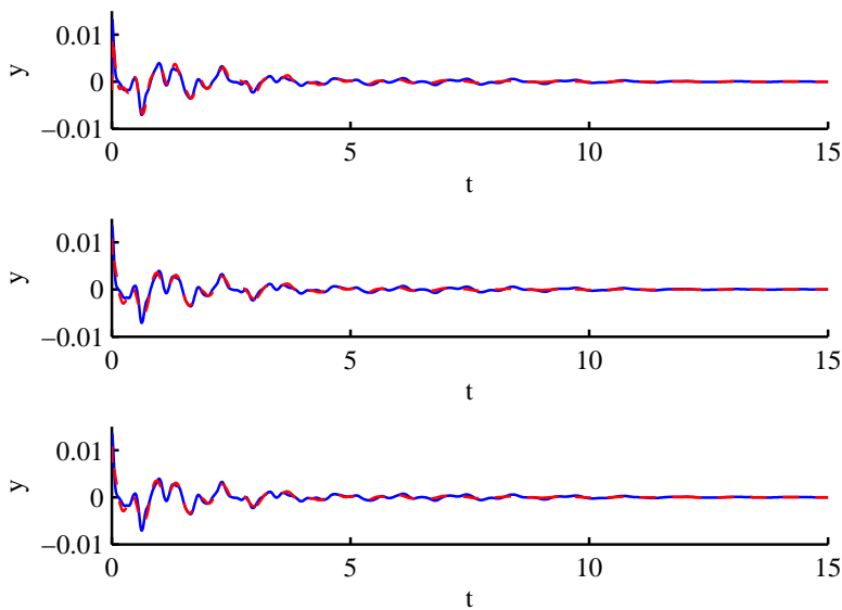
Figure 4.4: Impulse response from reduced-order models.
